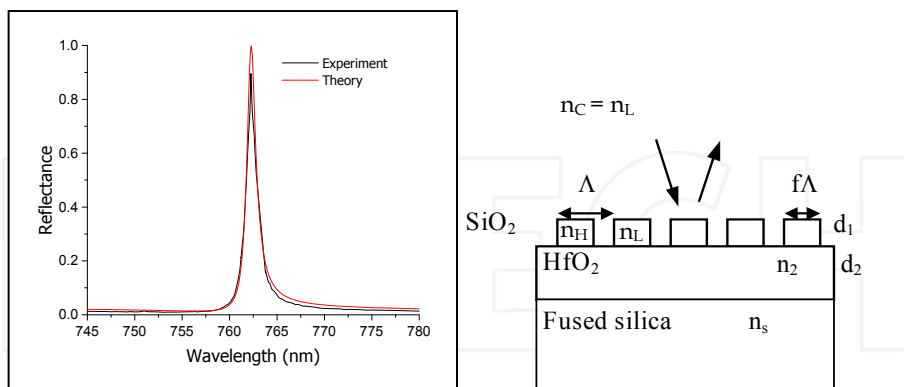
Fig. 2. Comparison between experiment and theory for a dielectric resonance element. The parameters used for the theoretical curve fit are close to the nominal values; they are n_C=1.0 , n_H=1.454 (SiO 2 ), n_2=1.975 (HfO 2 ), n_s=1.454 , d_1=135 nm, f=0.58 , d_2=208 nm, \Lambda=446 nm, normal incidence. Rigorous coupled-wave analysis (RCWA) is used for the computations (Gaylord & Moharam, 1985).
