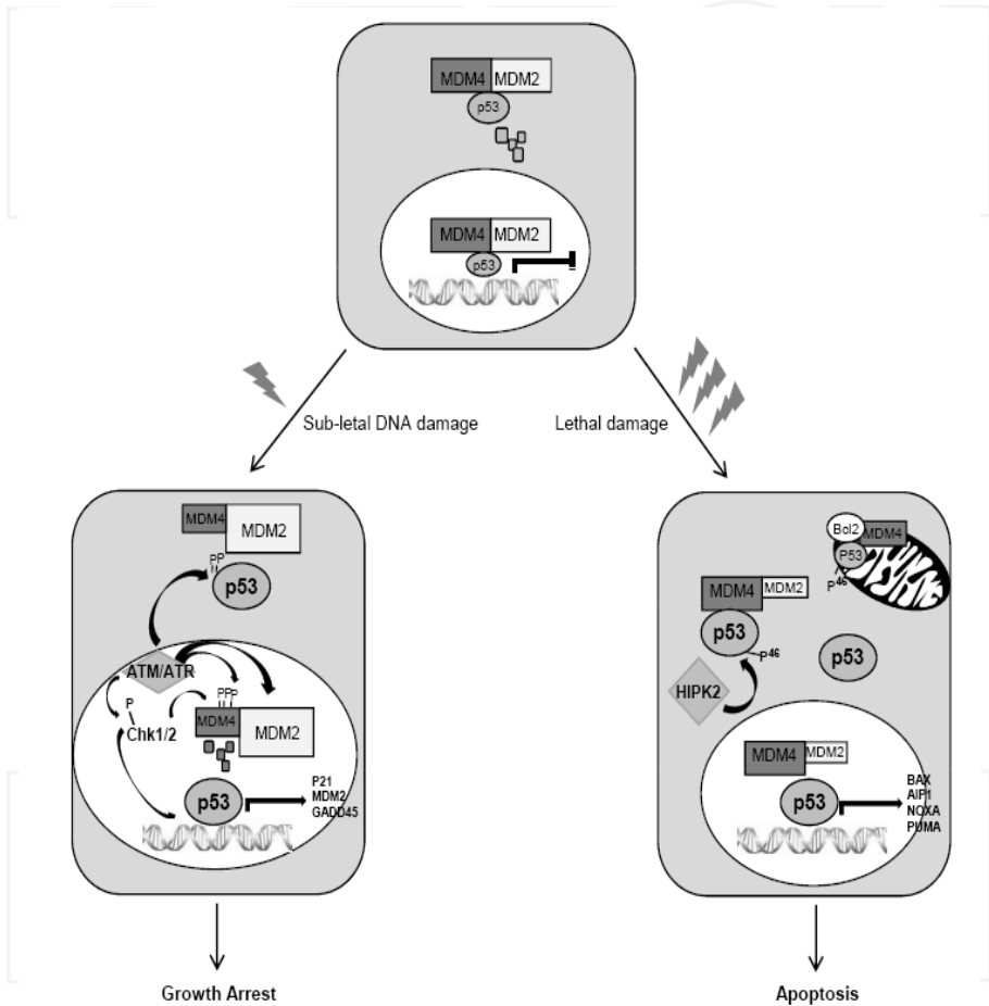
Fig. 3. P53 network following different DNA damages.
