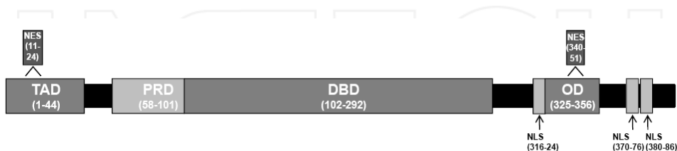
Fig. 1. P53 protein domains. TAD=Trans-Activation domain; PRD=Proline-Rich domain; DBD=DNA-binding domain; OD=Oligomerization domain; NES=Nuclear export signal; NLS=Nuclear localization signal.
