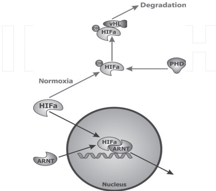
Fig. 1. Graphical representation of the HIF pathway during normoxic and hypoxic conditions. In normoxia (grey arrows) PHD hydroxylates HIF- \alpha , which then binds to vHL, leading to its proteosomal degradation. In hypoxia (black arrows) HIF- \alpha enters the nucleus, forms a dimer with ARNT, which then binds to DNA, leading to gene transcription activation [Gourvas et al., 2010].
