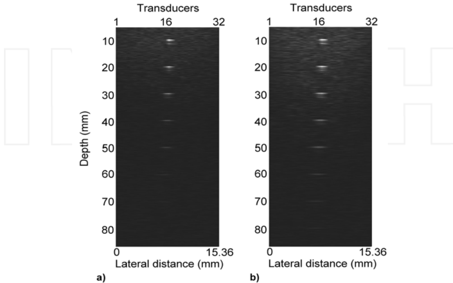
Fig. 15. 2D ultrasound images of tissue mimicking phantom: a) using STA method; b) using multi-element STA method
