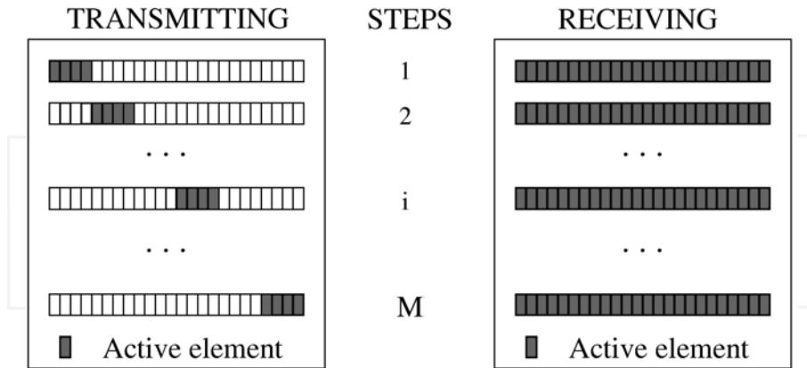
Fig. 3. Transmitting and receiving in multi-element STA method
