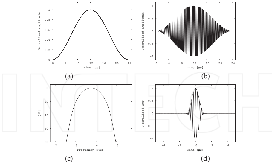
Fig. 3. Chirp signal with Hanning window. Time duration is 24 \mu s , and frequency is 2.5–5 MHz. (a) Window shape, (b) time domain, (c) frequency spectrum, and (d) ACF (solid line) and its envelope (dashed line).
