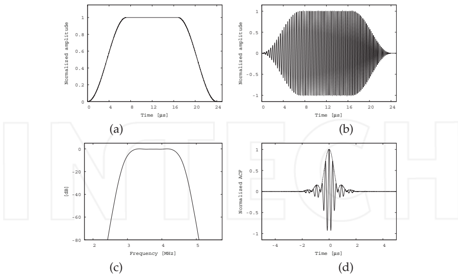
Fig. 4. Chirp signal with partial Hanning window ( d=0.3 ). Time duration is 24 \mu s , and frequency is 2.5–5 MHz. (a) Window shape, (b) time domain, (c) frequency spectrum, and (d) ACF (solid line) and its envelope (dashed line).
