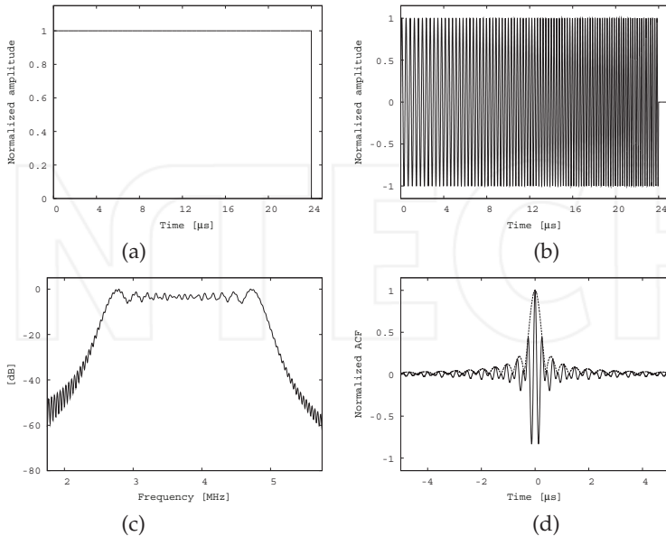
Fig. 2. Chirp signal with rectangular window. Time duration is 24 \mu s , and frequency is 2.5–5 MHz. (a) Window shape, (b) time domain, (c) frequency spectrum, and (d) ACF (solid line) and its envelope (dashed line).
